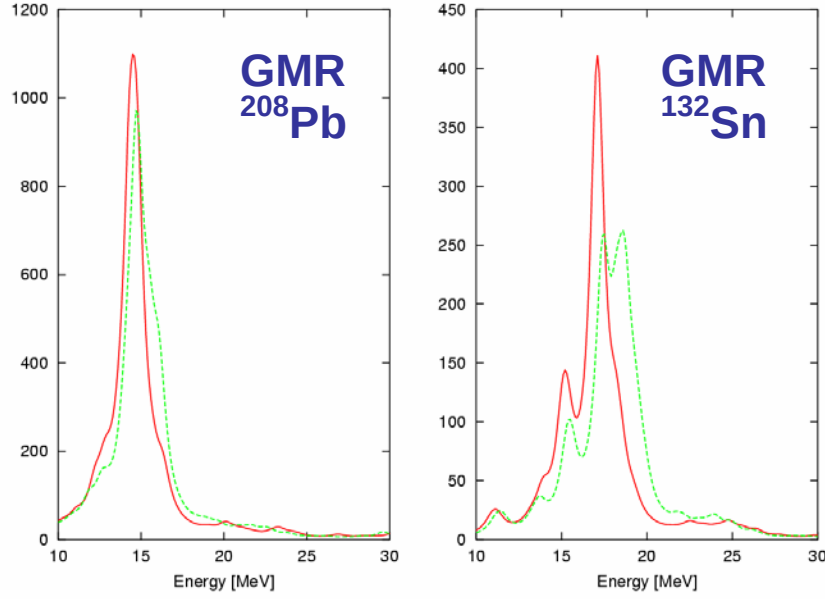
Figure A.3: Calculated strength function for the isoscalar Giant Monopole Resonance for ^{208}\text{Pb} (left) and ^{132}\text{Sn} (right).
