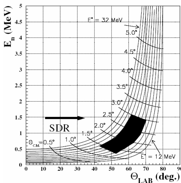
Figure B.16: Kinematical quantities and domains for the ^{132}\text{Sn}(p,n) reaction at 400 MeV per nucleon.
