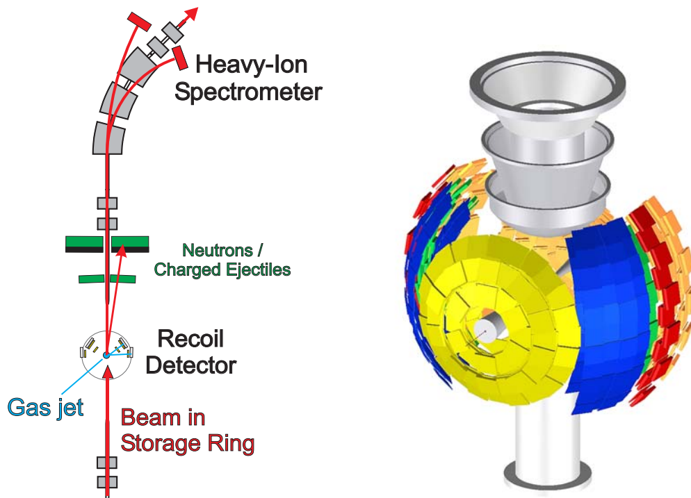
Figure 1: Schematic view of the EXL detection systems. Left: Set-up built into the NESR storage ring. Right: Target-recoil silicon detector and gas-jet target.
