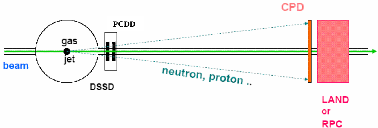
Figure B.17: Schematic view of the ejectile detector system.
