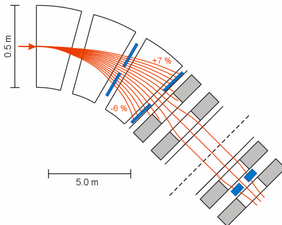
Figure B.19: Trajectories calculated for ions of different magnetic rigidity in part of the first 90° bending section behind the NESR internal target, three dipole magnets followed by four quadrupole magnets are shown. The mid plane of the bending section is indicated (dashed line). Trajectories are shown in steps of 1% relative difference in magnetic rigidity. In blue color, the detector positions are indicated.
