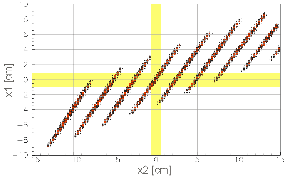
Figure B.20: Separation of uranium charge states (from left to right: U^{92+} to U^{84+} ) obtained with two tracking detectors in pockets in front and behind the third dipole of the arc. A wide beam emerging from the target with spot size of \pm 5 mm and of \pm 5 mrad divergence was assumed. The two yellow bars indicate the space that has to be free of matter for the circulating beam.
