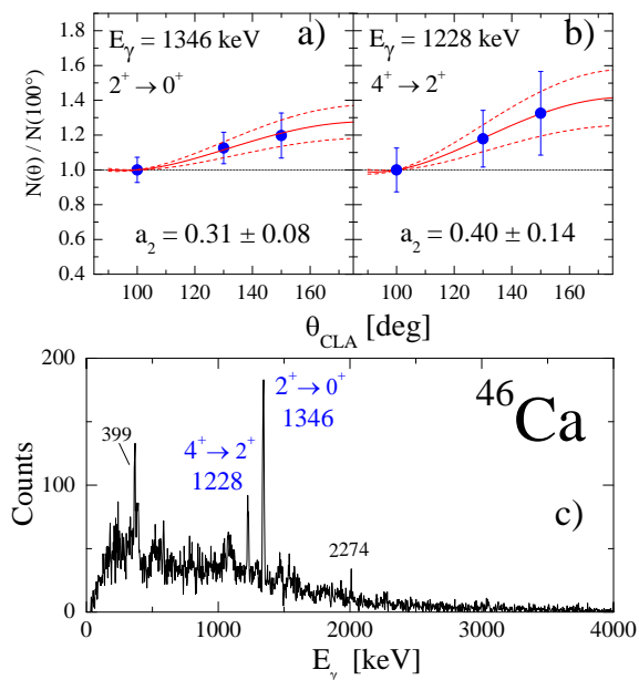
FIG. 4: (Color online) Bottom panel: Gamma spectrum (with 3 keV/ch) measured in coincidence with ^{46}\text{Ca} ions detected in PRISMA. Panel a) and b): Angular distribution of the 2^+ \rightarrow 0^+ and 4^+ \rightarrow 2^+ transitions at 1346 and 1228 keV, respectively. The solid lines are the fit by the angular distribution function W(\theta) = 1 + a_2 P_2(\cos\theta) , while the dotted lines give the uncertainty in W(\theta) . The extracted a_2 values are given in each panel.
