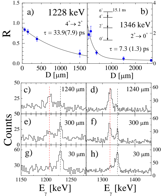
FIG. 22: (Color online) Bottom panels: Gamma spectra of ^{46}\text{Ca} , at different target-to-degrader distances, showing the 4^+ \rightarrow 2^+ transition at 1228 keV (left) and the 2^+ \rightarrow 0^+ decay at 1346 keV (right), together with their Doppler shifted components. Top panels: Interpolations of the ratio R , providing the lifetime \tau of the 4^+ and 2^+ states.
