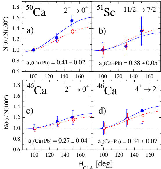
FIG. 7: (Color online) Comparison between the angular distributions of known E2 transitions of ^{46,50}\text{Ca} and ^{51}\text{Sc} nuclei, as follows from the analysis of the Ca+Ni (filled circles) and Ca+Pb data (open circles). Solid and dashed lines are the corresponding fits of the data by the angular distribution function W(\theta) , which in the case of Ca+Pb provide the a_2 values given in each panel.
