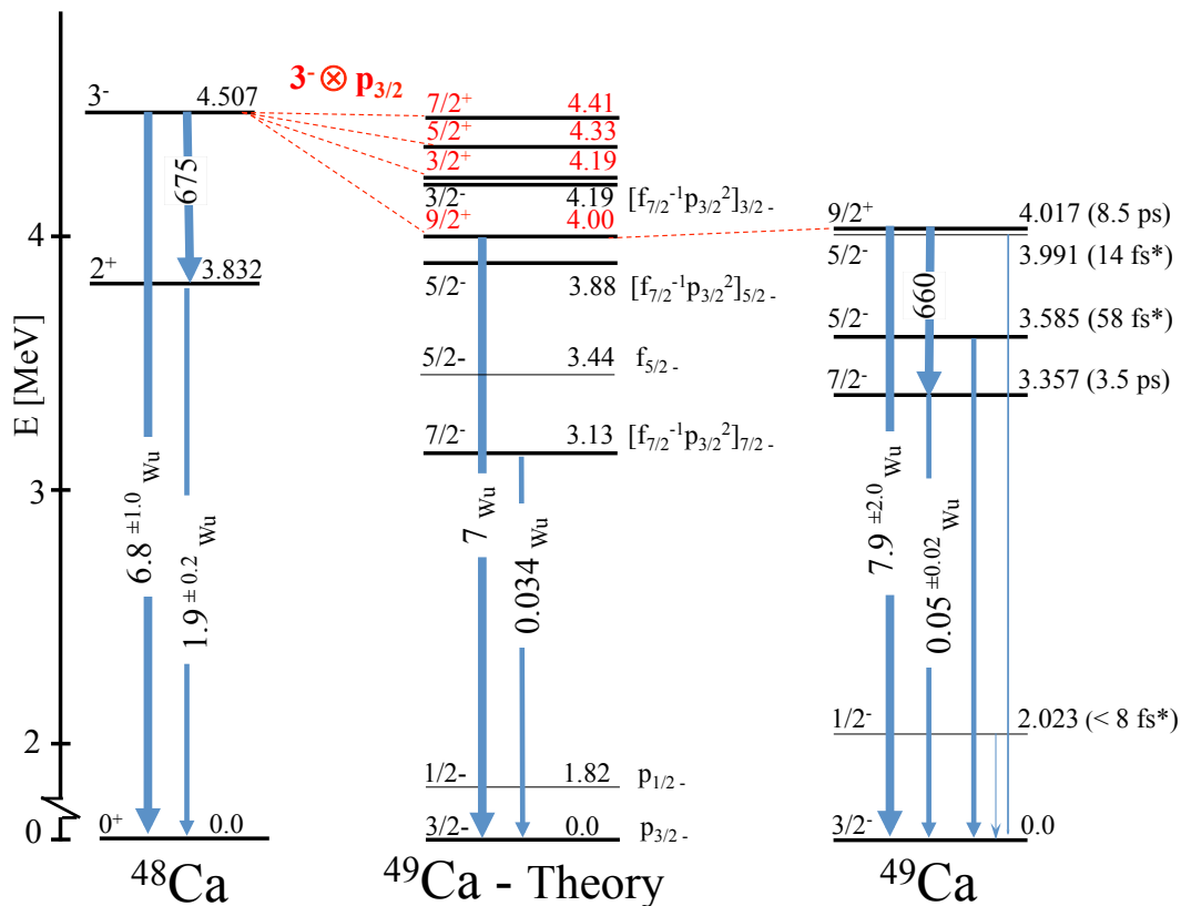
FIG. 10: (Color online) Right: Decay scheme of ^{49}\text{Ca} , as observed in this work. Right labels give the energy of the level (taken from Refs. [15, 53]) and its lifetime (in parenthesis), as deduced from this work. Stars refer to values taken from Ref. [53]. Thick arrows indicate the decay from particle-phonon coupled states, very thin arrows from states of single particle nature (also indicated by thin lines). Center: calculated levels of ^{49}\text{Ca} . Positive parity states are obtained with the particle-vibration coupling model discussed in Sec. IV C, employing the SkX Skyrme interaction (as discussed in the main text). Negative parity states are calculated by the full fp shell model of Ref. [43], with dominant configurations given on the right side of each level. Left: experimental 2^+ and 3^- levels of ^{48}\text{Ca} . The B(E\lambda) strengths of the relevant \gamma transitions are reported on the arrows in Weisskopf units (Wu) (from Refs. [36, 38] and present work). (Adapted from Ref. [19]).
