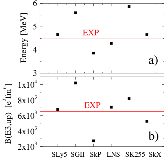
FIG. 16: (Color online). Energy (top) and B(E3, \text{up}) (bottom) of the 3^- state of ^{48}\text{Ca} , as obtained from RPA calculations using different Skyrme forces. The horizontal lines correspond to the experimental values.
