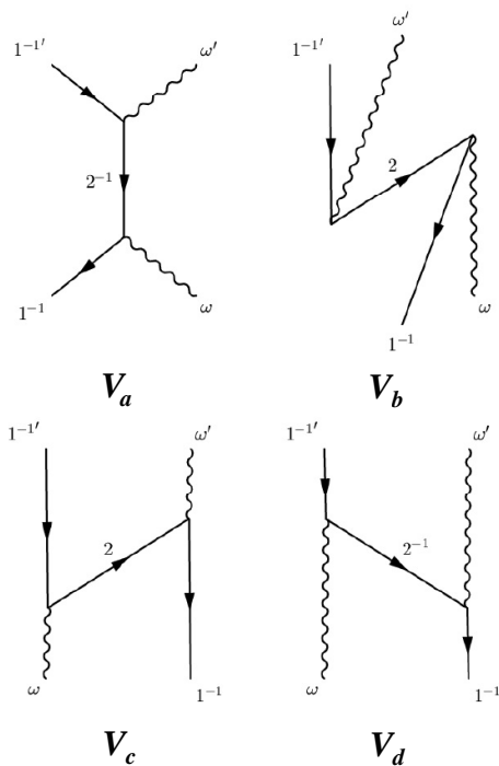
FIG. 27: The same as Fig. 26 in the case of a multiplet made up with a hole coupled to a vibration.
