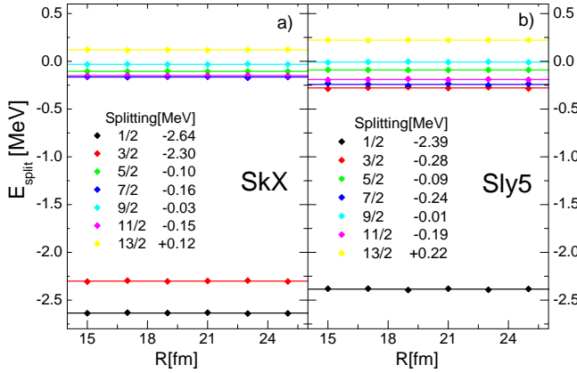
FIG. 19: (Color online) Energy splitting of the 3 \otimes f_{7/2}^{-1} multiplet of ^{47}\text{Ca} for different values of the box dimension R adopted in the Hartree-Fock calculation with the SkX (left) and SLy5 (right) interactions. The average energy splitting for each multiplet member is given in the legend.
