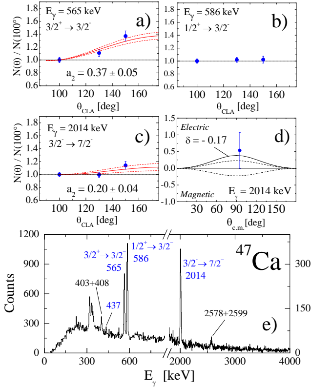
FIG. 12: (Color online) Bottom: Gamma spectrum (with 3 keV/ch) measured in the Ca+Ni experiment, in coincidence with ^{47}\text{Ca} ions detected in PRISMA. Note that above 1800 keV the scale of the y axis is given on the right. Blue labels indicate transitions studied in details in this work. Panels a), b) and c): angular distributions of the 565-, 586- and 2014-keV lines, respectively. The a_2 coefficients are indicated in each panel, except for the 586-keV transition, which is isotropic, being generated by a 1/2^+ state. Panel d) shows the polarization analysis of the 2014-keV \gamma -ray. Symbol refers to data, dotted lines to pure electric/magnetic quadrupole transitions. A mixing with octupole component with \approx 3\% probability ( \delta = -0.17 ) is also indicated by solid line (see text for details).
