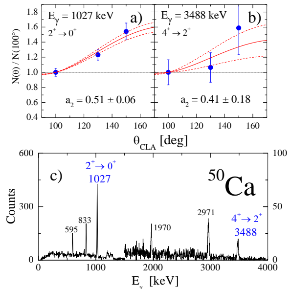
FIG. 3: (Color online) Bottom panel: Gamma spectrum (with 3 keV/ch) measured in coincidence with ^{50}\text{Ca} ions detected in PRISMA. Note that above 1500 keV the scale of the y axis is given on the right. Panel a) and b): Angular distributions of the 2^+ \rightarrow 0^+ and 4^+ \rightarrow 2^+ transitions at 1027 and 3488 keV, respectively. The solid lines are the fit by the angular distribution function W(\theta) = 1 + a_2 P_2(\cos\theta) , while the dotted lines give the uncertainty in W(\theta) . The extracted a_2 values are given in each panel.
