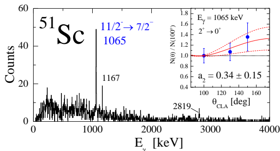
FIG. 5: (Color online) Gamma spectrum (with 3 keV/ch) measured in coincidence with ^{51}\text{Sc} ions detected in PRISMA. The inset of the figure shows the angular distribution of the 11/2^- \rightarrow 7/2^- transition at 1065 keV. The solid line are the fit by the angular distribution function W(\theta) = 1 + a_2 P_2(\cos\theta) , while the dotted lines give the uncertainty in W(\theta) . The extracted a_2 value is given in the inset.
