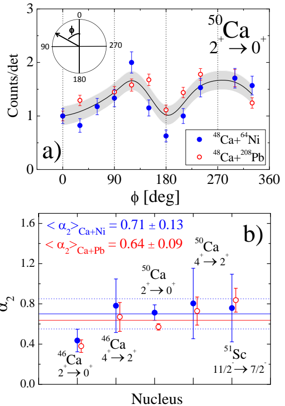
FIG. 6: (Color online) Bottom panel: Fraction \alpha_2 of full spin alignment obtained from the experimental angular distributions of known stretched E2 transitions, following the decay of ^{46,50}\text{Ca} and ^{51}\text{Sc} nuclei, populated in the ^{48}\text{Ca} + ^{64}\text{Ni} and ^{48}\text{Ca} + ^{208}\text{Pb} reactions (full and empty circles, respectively). The corresponding average values \alpha_2 = 0.71 \pm 0.13 and 0.64 \pm 0.09 are indicated by solid lines. Dashed lines indicate the uncertainty in the Ca+Ni analysis. Top panel: anisotropy of the 2^+ \rightarrow 0^+ transition of ^{50}\text{Ca} , as a function of the polar angle \phi at \theta_{CLA} = 100^\circ , as measured for both reactions. The average between the two reactions is given by the solid line, while the corresponding uncertainty is indicated by the shaded band. The inset shows the coordinate systems used to define the polar angle \phi .
