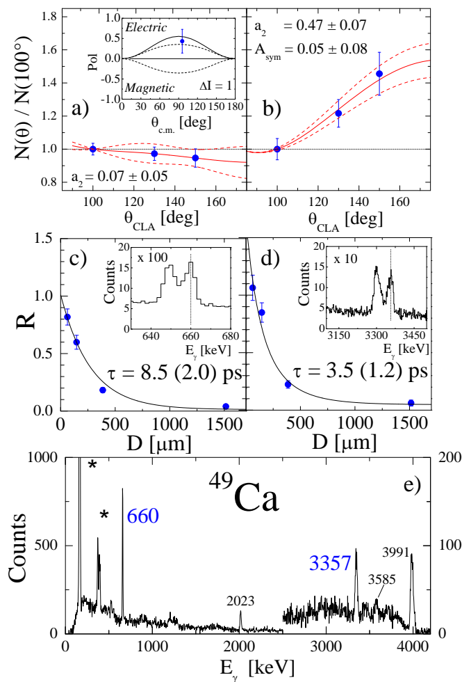
FIG. 9: (Color online) Bottom panel: Gamma spectrum (with 3 keV/ch) measured in coincidence with ^{49}\text{Ca} ions in the Ca+Ni experiment. Contaminant lines from the binary partner ^{63}\text{Ni} are marked by stars. Note that above 2500 keV the scale of the y axis is given on the right. Top panels (a) and b): Angular distribution of the 660- and 3357-keV transitions, providing a_2 parameters equal to 0.07 \pm 0.05 and 0.47 \pm 0.07 , respectively. The inset of panel a) gives the polarization of the 660-keV \gamma ray, in comparison with prediction for a pure electric or magnetic dipole (dashed lines). The solid line corresponds to the expected values for an electric dipole with a 4% quadrupole component. For the 3357-keV transition the asymmetry value is given. Middle panels c) and d): experimental ratio R = I_{After}/I_{660} versus the effective target-to-degrader distances, for the 660- and 3357-keV lines, as determined in the Ca+Pb experiment. The inset of each panel shows the two components structure of each transition, as observed in the \gamma spectrum obtained by summing the plunger measurements at all distances. The dashed lines indicate the position of the components corresponding to the decay after the degrader (adapted from Ref. [19]).
