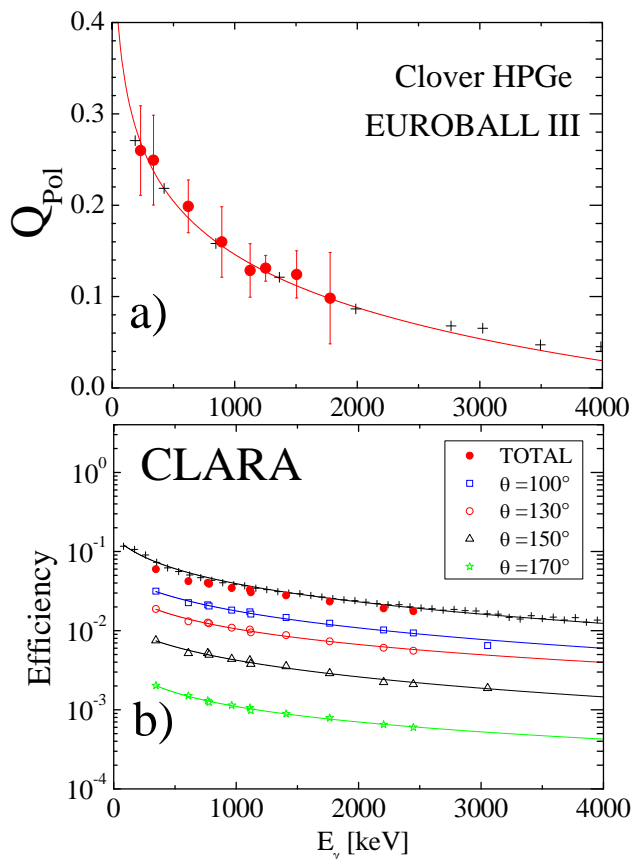
FIG. 1: (Color online) Bottom panel: Absolute efficiency of the CLARA Ge array. Cross symbols refer to simulation calculations for the complete geometry of 25 clover detectors. Filled circles are the experimental measurements for the geometry of 23 detectors, used in the experiments, as obtained with an ^{152}\text{Eu} source. The measured efficiencies of the detector rings at \theta_{CLA} = 100^\circ , 130^\circ , 150^\circ and of the additional detector at 170^\circ are also shown by open symbols. Top panel: the polarization sensitivity Q of the clover detectors [26], as obtained from simulation calculations (crosses) and experimental measurements from known transitions (circles).
