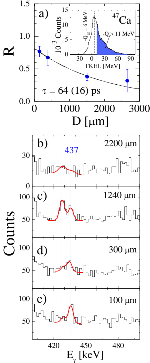
FIG. 14: (Color online) Bottom panels: gamma spectrum of ^{47}\text{Ca} at different target-to-degrader distances showing the 437 keV transition (black dotted line) and its Doppler shifted component at about 430 keV (red dotted line). The spectra have been constructed with the condition \text{TKEL} = -Q > 11 MeV, as shown in the inset of panel a). The red lines represent the Gaussian fit for the high- and low-energy components (corresponding to the decay after and before the degrader, respectively), used to determine the ratio R given in panel a).
