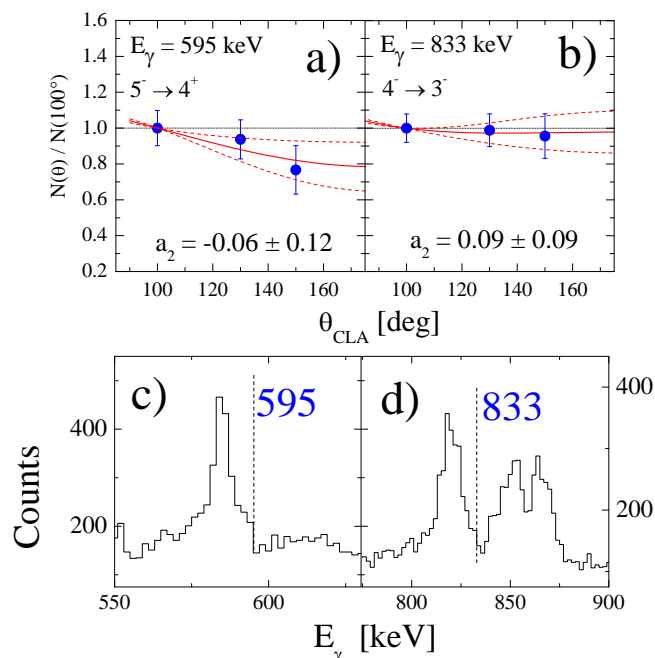
FIG. 24: (Color online) ^{50}\text{Ca} : Panel a) and b): angular distributions of the 595 and 833-keV lines, as obtained from the Ca+Ni data. The a_2 coefficients reported in the panels are compatible with dipole transitions between the indicated levels, with small admixture of quadrupole decays ( \approx 1.5\% and 6\% , respectively). Panel c) and d): \gamma spectrum of ^{50}\text{Ca} summed over all target-to-degrader distances used in the Ca+Pb plunger experiment. The energy regions relevant for the Doppler shift analysis of the 595 and 833-keV lines are displayed, with dashed lines indicating the expected position for the component corresponding to the decay after the degrader.
