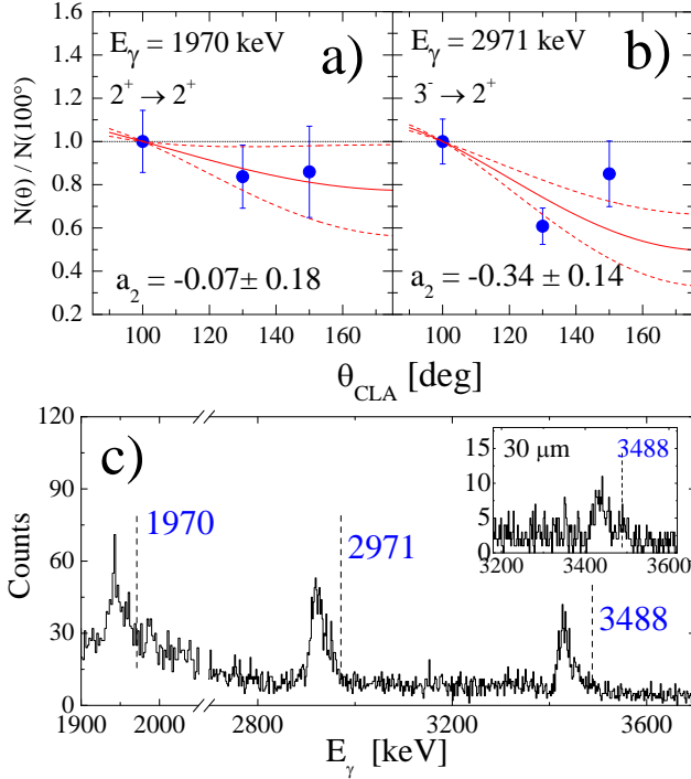
FIG. 25: (Color online) ^{50}\text{Ca} : Panel a) and b): angular distributions of the 1970 and 2971-keV lines, as obtained from the Ca+Ni data. The a_2 coefficients reported in the panels are compatible with dipole transitions between the indicated levels, with admixture of quadrupole decays of the order of \approx 16\% and < 1\% , respectively. Panel c): \gamma spectrum of ^{50}\text{Ca} summed over all target-to-degrader distances used in the Ca+Pb plunger experiment. The energy region relevant for the Doppler shift analysis of transitions at 1970, 2971 and 3488 keV is displayed, with dashed lines indicating the positions of the high-energy components corresponding to the decay after the degrader. The inset shows the 3488-keV line measured at the shortest distance of 30 \mu\text{m} , with indication of a very weak high-energy component.
