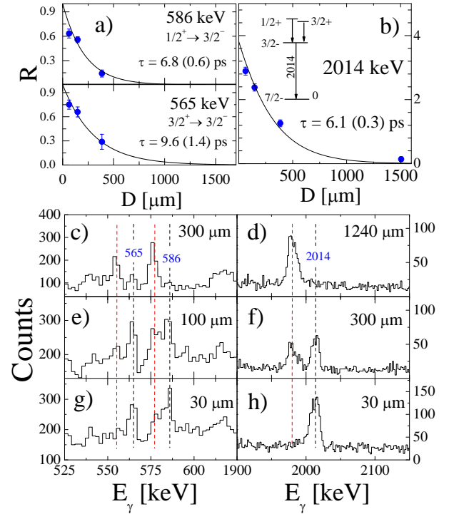
FIG. 13: (Color online) Doppler shift analysis of the 565-, 586- and 2014-keV lines of ^{47}\text{Ca} by the RDDS method. Top panels a) and b) show the fit of the intensity ratio R between the high-energy component (corresponding to the decay after the degrader) and the total intensity of the \gamma -decay line, as observed in the Ca+Pb experiment, at various target-to-degrader distances. In the case of the 2014-keV line, the feeding from the 1/2^+ and 3/2^+ states, deexciting by the 586- and 565-keV lines, has been taken into account. Left (right) panels c), e) and g) (d), f) and h)) show the regions of the \gamma -spectrum relevant for the Doppler shift analysis of the 586-, 565- and 2014-keV lines, respectively. Black (red) lines give the centroid positions of the components decaying after (before) the degrader.
