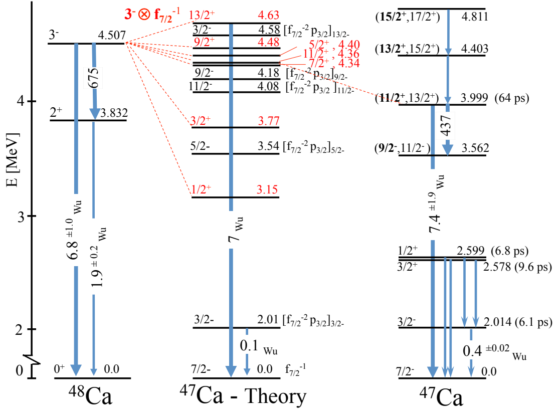
FIG. 11: (Color online) Right: Decay scheme of ^{47}\text{Ca} , as observed in this work. Right labels give the energy of the level (taken from Refs. [15, 53]) and its lifetime (in parenthesis), as deduced from this work. Thick arrows indicate the decay from states of particle-phonon nature. Center: calculated levels of ^{47}\text{Ca} . Positive parity states are obtained with the hole-phonon coupling model discussed in Sec. IV C, employing the SkX Skyrme interaction (as discussed in the main text). Negative parity states are calculated by the full fp shell model of Ref. [43], with dominant configurations given on the right side of each level. Left: experimental 2^+ and 3^- levels of ^{48}\text{Ca} . The B(E\lambda) strengths of the relevant \gamma transitions are reported on the arrows in Weisskopf units (Wu) (from Refs. [36, 38] and present work).
