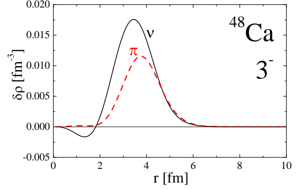
FIG. 17: (Color online). Transition densities of the 3^- state of ^{48}\text{Ca} , for neutrons and protons, obtained by RPA calculations with the SLy5 interaction.
