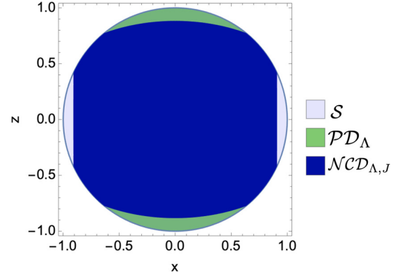
FIG. 4. Section at y = 0 of the Bloch sphere [light blue (light gray)] for an example of a nonpositive map \Lambda for which the noncontractivity domain \mathcal{NCD}_{\Lambda,J} [blue (dark gray)] is strictly included in the positive domain \mathcal{PD}_{\Lambda} [green (medium gray)]. This map acts on a Bloch vector \mathbf{r} = (x, y, z)^T as \mathbf{r} \mapsto (\lambda_x x, \lambda_y y, \lambda_z z)^T , with \lambda_x = \lambda_y = 1.1 and \lambda_z = 0.1 .
