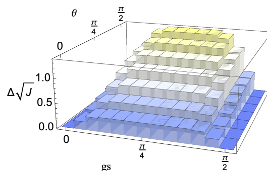
Figure 3. Plot of the l.h.s. of Equation (20) showing the revivals of the \text{QJSD}^{1/2} as a function of time and choice of initial system states. The reference time gt is fixed to be \pi/2 , i.e., after one full period of the evolution, while gs sweeps from 0 to \pi/2 . The initial pair of system states is given by \rho_S^1(0) = |+\rangle\langle +| and \rho_S^2(0) = |\theta\rangle\langle \theta| , as shown in Figure 2, with \theta ranging from 0 to \pi/2 , corresponding to the case of an orthogonal pair and maximizing the revivals.
