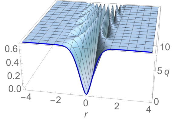
FIG. 2. Entropy of entanglement [see Eq. (81)] for a system-environment correlated state as in Eq. (73) with momentum distribution f(Q) and phase \theta(Q) as in Eq. (82), as a function of r and q ; the section for q = 0 (thick blue line) corresponds to the case where f(Q) is a single Gaussian peak, i.e., Eq. (80).
