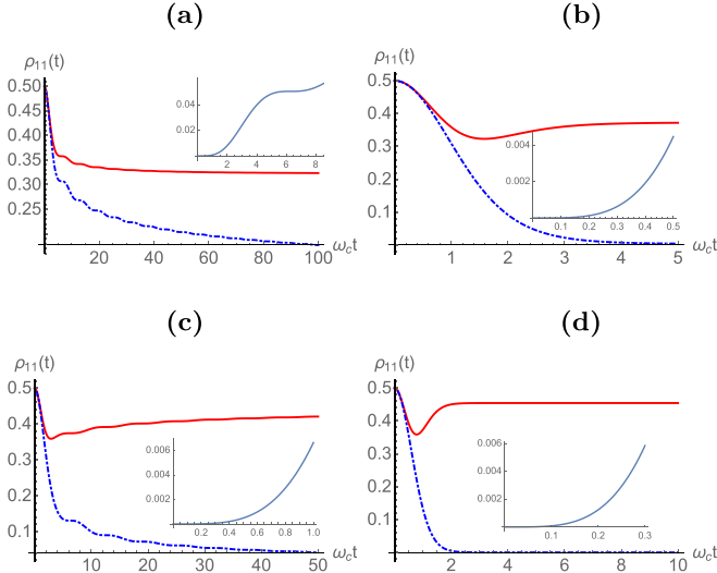
FIG. 7. Second-order APO (red solid line) and second-order TCL (blue dot-dashed line) solutions for \rho_{11}(t) as a function of time t , for the damped two-level system dynamics fixed by Eq. (83), with a spectral density as in Eq. (98) and an initial correlated global state as in Eq. (93), with C_0 = C_1 = 1/\sqrt{2} and the number of bosons in the mode with frequency \omega as in Eq. (99). The values of \gamma and N are (a) \gamma = 0.05 and N = 3 , (b) \gamma = 0.5 and N = 3 , (c) \gamma = 0.05 and N = 10 , and (d) \gamma = 0.5 and N = 10 . The inset shows the difference between the APO and TCL second-order solution in the short-time regime. In all panels, \omega_c/\nu = 100 and \zeta = 0 .
