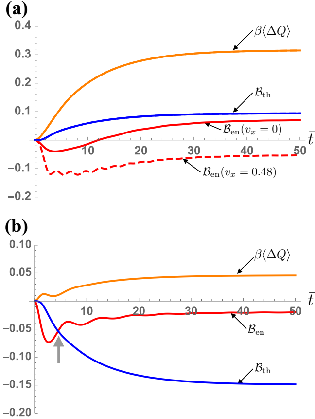
FIG. 1. Time evolution of the bounds \mathcal{B}_{en} and \mathcal{B}_{th} , and the mean dissipated heat \langle\Delta Q\rangle for several initial conditions. (a) We compare their time evolutions for two different initial conditions with the same population without coherence [ \mathbf{v}_1(0) = (0, 0, 0.28) : solid lines] and with coherence [ \mathbf{v}_2(0) = (0.48, 0, 0.28) : dashed lines]. Solid lines and dashed lines coincide for the mean dissipated heat (orange line) and the thermodynamic bound (blue line), whereas they diverge for the entropic bound (red lines). (b) We plot their time evolutions for another initial state different from the solid lines in (a) in their initial populations [ \mathbf{v}_3(0) = (0, 0, -0.5) ]. The gray arrow in the panel indicates crossover of \mathcal{B}_{en} and \mathcal{B}_{th} . Their time evolutions differ from the solid lines in (a), thus the three quantities explicitly depend on the initial populations. In the numerical calculations, we set the parameters to \lambda = 0.1 , \Omega = 0.4 , and \beta = 1 .
