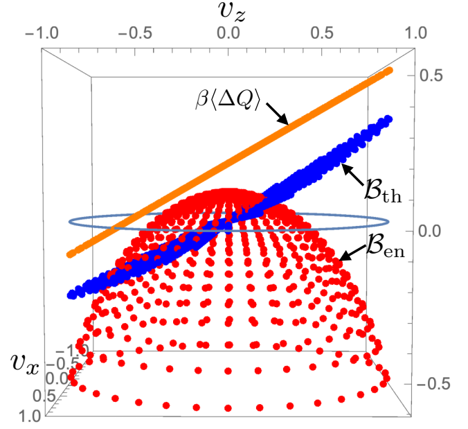
FIG. 2. Dependence of the relative tightness on the initial state. The bounds and the mean dissipated heat are calculated for 720 systematically chosen initial states. The initial condition is chosen by changing v_x(0) and v_z(0) with v_y(0) = 0 to focus on the dependence on initial coherence and initial population. The orange points represent heat, the blue points represent the thermodynamic bound, and the red points represent the entropic bound. The purple circle indicates the surface of the Bloch sphere with v_y = 0 . In the numerical calculations, we set the parameters to \lambda = 0.1 , \Omega = 0.4 , and \beta = 1 (same as in Fig. 1).
