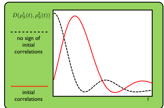
FIG. 7. The behavior of the trace distance with and without initial correlations. If the trace distance between two states, prepared such that \rho_{SE}^2(0) = (\Lambda \otimes I) \rho_{SE}^1(0) , never exceeds its initial value (dashed black line), the dynamics does not witness initial correlations. If, on the other hand, the trace distance for such pair of states increases above the initial value (solid red line), we can conclude the presence of initial correlations.
