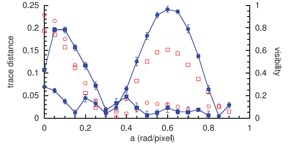
FIG. 2. (Color online) Trace distance and visibility as a function of the experimental evolution parameter a , the two quantities are related through Eq. (6). Full circles describe the trace distance between \rho_s^1(a) , i.e., f(n - n_2) = 0 , and \rho_s^2(a) with f(n - n_2) = \sin[\lambda(n - n_2)] , \lambda = -0.6 \text{ rad/pixel} . Full squares describe the trace distance between \rho_s^1(a) and \rho_s^2(a) with f(n - n_2) = \tau(n - n_2) , \tau = 0.1 \text{ rad/pixel} . Lines are a guide for the eye. Empty circles refer to visibility with the choice f(n - n_2) = 0 , whereas empty squares refer to the case in which initial correlations are introduced through the phase function f(n - n_2) = \sin[\lambda(n - n_2)] . For the visibility, the uncertainties are within the symbols.
