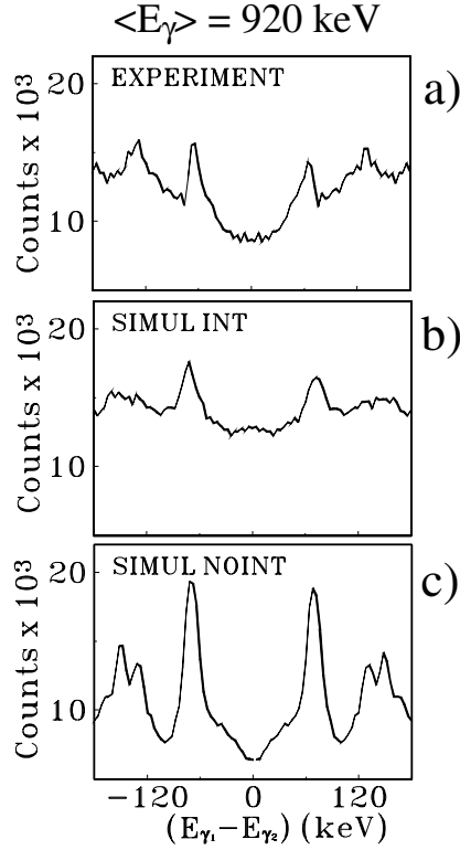
Figure 15. Perpendicular cuts, 60 keV wide, at the average transition energy \langle E_\gamma \rangle = 920 \text{ keV} , on experimental (a) and simulated (b) and (c) \gamma - \gamma coincidence matrices of ^{168}\text{Yb} . The simulated spectra have been based on cranking calculations including (b) or not (c) a two-body residual interaction of surface delta type [10, 15]. The most intense discrete transitions were subtracted from the right-hand side of the spectra in all cases (adapted from [15]).
