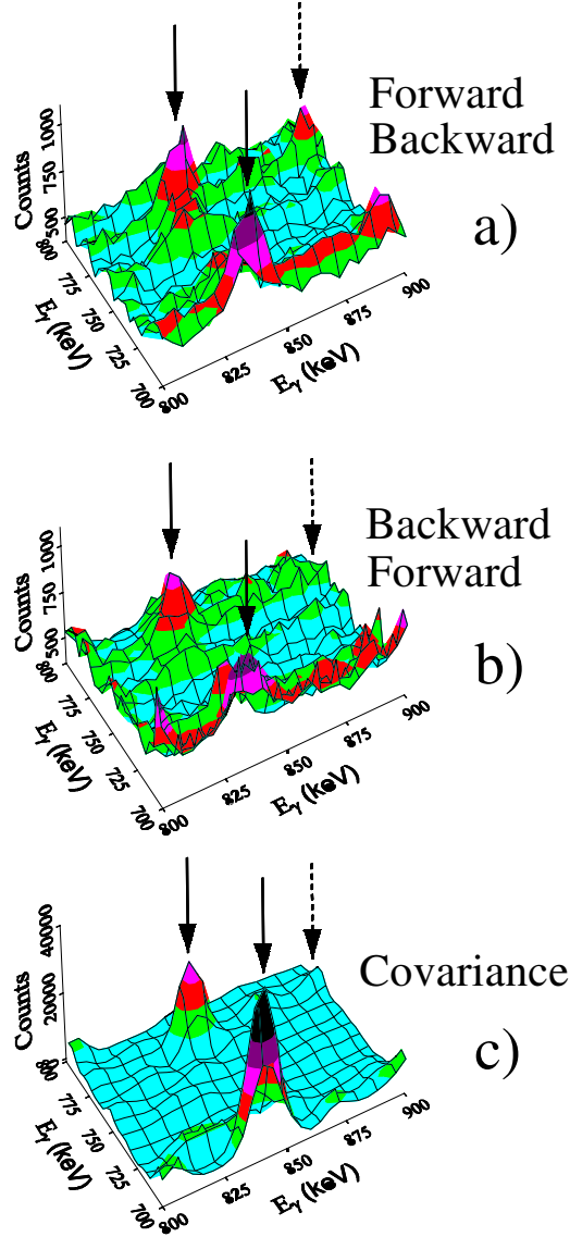
Figure 19. Sections of 2D coincidence matrices having on the x and y axes the \gamma -ray energies detected at forward and backward angles (a), and vice versa (b), in a backed target experiment on ^{164}\text{Yb} [21]. The covariance spectrum between the two previous distributions, defined according to equation (7), is shown in panel (c). The arrows indicate structures which are common (full) or not (broken) to the (a) and (b) distributions.
