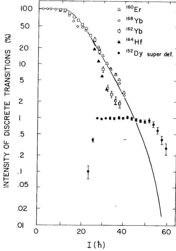
Figure 41. Discrete line intensities normalized to the 2^+ \rightarrow 0^+ ground state transition, for the well deformed nuclei ^{160}\text{Er} , ^{168}\text{Yb} and ^{164}\text{Hf} and for the SD band of ^{152}\text{Dy} . The intensities plotted are the sum of all observed discrete lines at the given spin. The full curve shows the calculated discrete line intensity for the case of ^{168}\text{Yb} (adapted from [86]).
