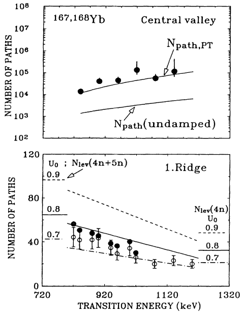
FIG. 3. The empirically determined values N_{\text{path}}^{(2)} . In the upper part, the values of N_{\text{path}}^{(2)} associated with coincidences with energies E_{\gamma_1} = E_{\gamma_2} (valley) are shown. In the lower part, the corresponding results associated with the first ridge are plotted with open circles. Shown by solid circles is the result obtained by adding the number of removed discrete peaks to the value of N_{\text{path}}^{(2)} . Theoretical calculations carried out making use of Eq. (8) and of different values for U_0 are shown. Equal composition of intensity from the 4n and 5n reaction channels has been assumed for the lower transition energies, with a linear decrease of the 5n component up to 1200 keV. Also shown is the actual number of levels N_{\text{lev}} below U_0 , obtained by integrating the level density up to U_0 .
