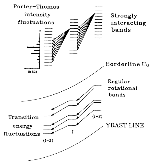
FIG. 1. Schematic representation of the \gamma -decay pattern of excited, rapidly rotating nuclei in the plane of excitation energy and spin.
