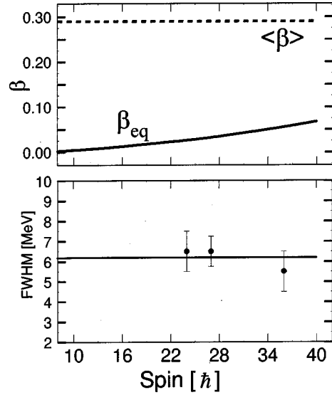
FIG. 5. The deduced GDR width at \langle T \rangle = 1.3 MeV as a function of angular momentum in comparison with the thermal shape fluctuation predictions described in the text (full line). In the top part of the figure the equilibrium deformation (that minimizes the Free energy) and the average deformation of ^{194}\text{Hg} are shown.
