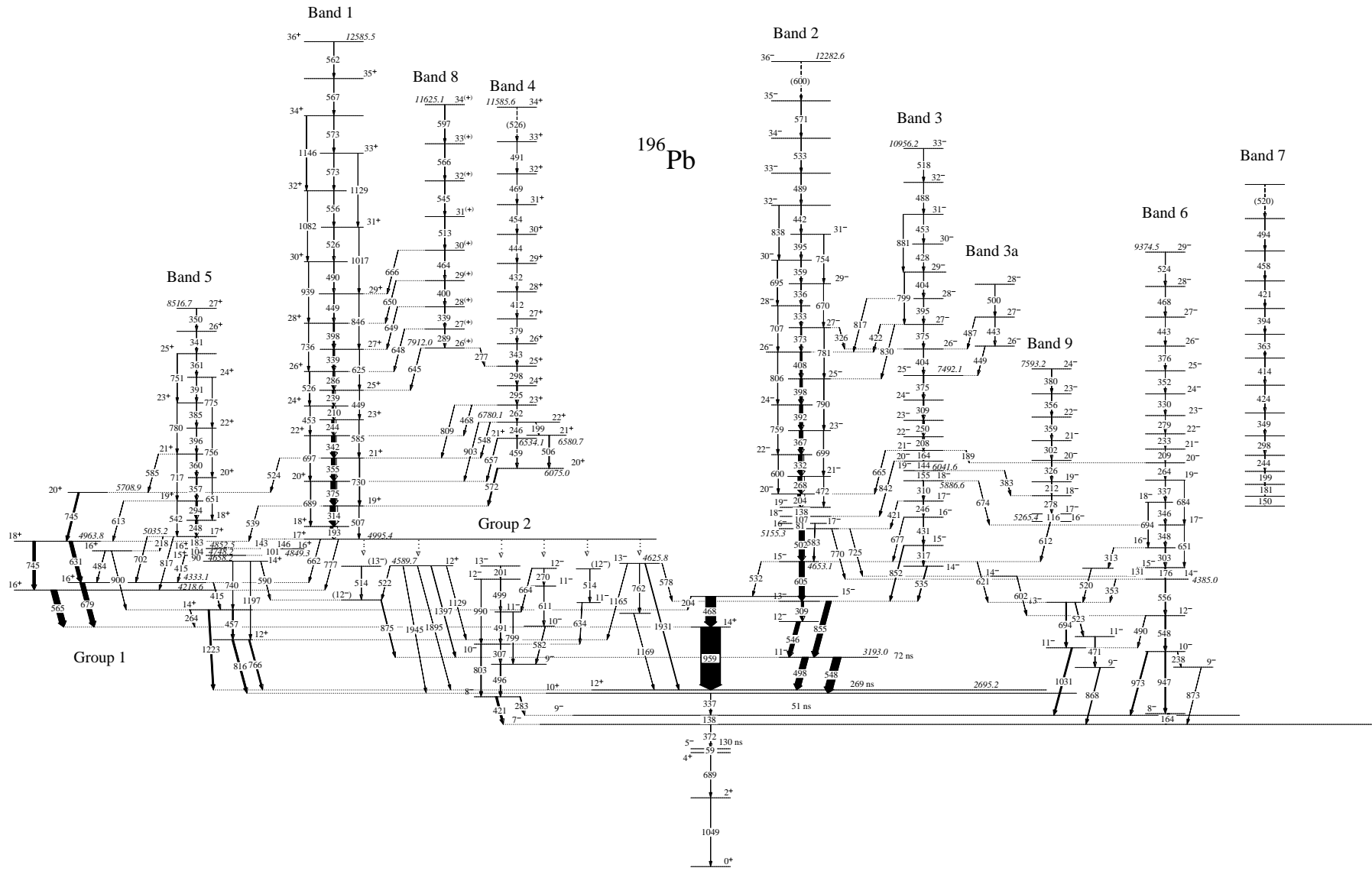
Figure 9.6: Partial level scheme of ^{196}\text{Pb} [277].
