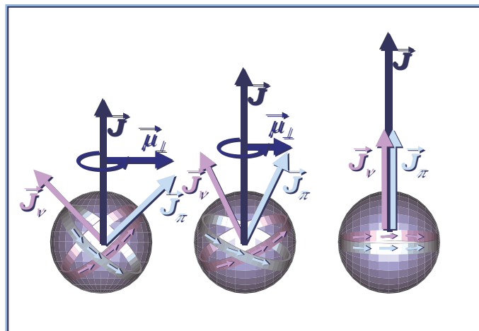
Figure 9.1: Schematic illustration of the shears effect in magnetic rotation bands [256].
