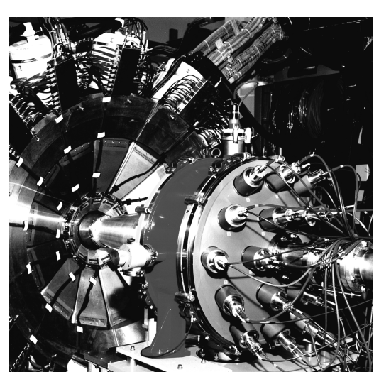
Figure 11.11 : The Recoil Filter Detector (RFD) coupled to EUROBALL.
