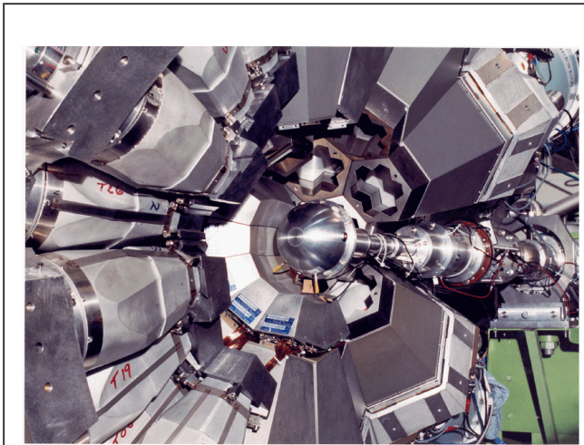
Figure 11.10: Plunger mounted in EUROBALL IV
