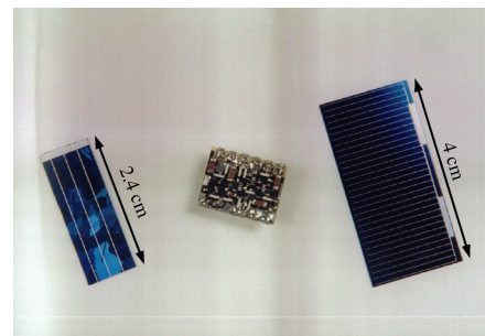
Figure 11.16: picture of two photovoltaic cells and one preamplifier.
