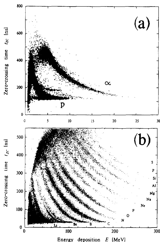
Fig. 6. Test of the zero-crossing technique without external time reference for p- \alpha and heavy-ion discrimination: The t_{ZC} - E plots were measured (a) in the reaction 150 MeV ^{36}\text{Ar} + \text{Ni} , \theta_{lab} = 110^\circ , U_D = 80 V, trigger rate \approx 1 kHz; (b) in the reaction 510 MeV ^{36}\text{Ar} + [\text{Ni} + \text{Al} + \text{C}] , \theta_{lab} = 25^\circ , U_D = 80 V, trigger rate \approx 0.5 kHz. Note the isotope resolution in the element branches. The E scales were calibrated assuming a linear dependence of the pulse height on the energy deposition.
