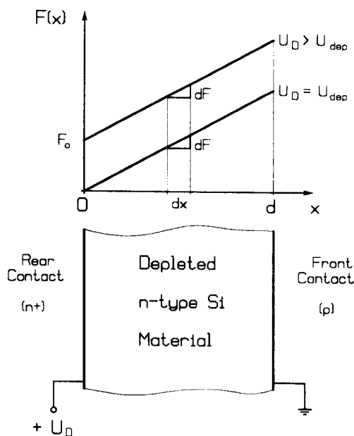
Fig. 8. Definition of the x axis and sketch of the electric field distribution in a reversed n-type Si detector: A homogeneous resistivity – resulting in a homogeneous space-charge density of the depleted silicon, and thus in a constant field gradient – is assumed. A maximum of dF(x)/(F \cdot dx) is obtained if the detector bias U_D equals the depletion voltage, U_{dep} .
