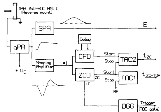
Fig. 2. Block scheme of the electronics used in our test: qPA – charge-sensitive preamplifier (IV69B, HMI Berlin), SPA – spectroscopy amplifier (Canberra 2022D), shaping amplifier – see text, CFD – constant-fraction discriminator (ORTEC 935), ZCD – zero-crossing discriminator with level discriminator (LD) and zero-crossing (ZC) outputs as described in Ref. [9], TAC1, TAC2 – time-to-amplitude converters (ORTEC 566/567), DGG – delay and gate generator (ORTEC GG8010), RF – cyclotron RF signal (used as TOF-start reference). * Inspection point (see Fig. 3).
