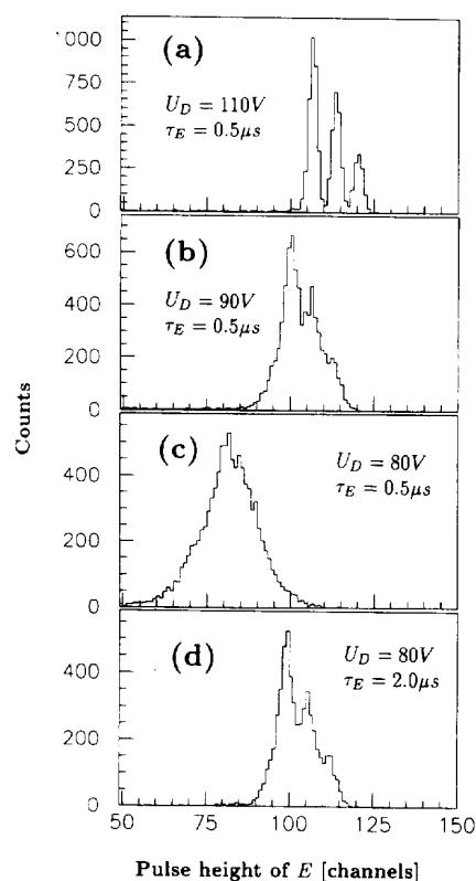
Fig. 9. Calibration spectra of a mixed ^{239}\text{Pu} – ^{241}\text{Am} – ^{244}\text{Cm} \alpha source, measured for different bias voltages U_D and with different shaping-time constants \tau_E of the spectroscopy amplifier generating the E signal (see Fig. 2). The peak shift is due to the ballistic deficit which increases strongly with decreasing bias voltage.
