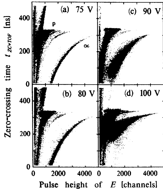
Fig. 4. Zero-crossing technique with external time reference, applied to proton–alpha discrimination: The t_{\text{ZC}+\text{TOF}}-E correlation, measured in the reaction 150 MeV ^{36}\text{Ar} + \text{Ni} with a detector at \theta_{\text{lab}} = 110^\circ (count rate \approx 1 kHz), allows excellent p– \alpha discrimination. A variation of the detector bias from 75 V (a) to 100 V (d) demonstrates that best resolution is obtained with a low bias (see text). The discontinuity of the alpha and proton branches in the scatterplots is due to the limited time range for t_{\text{ZC}+\text{TOF}} , given by the repetition rate of the beam bunches.
