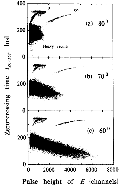
Fig. 5. Test of the count-rate dependence and the influence of scattered projectiles or recoiled target nuclei on the particle discrimination: The scatterplots were measured in the reaction 150 MeV ^{36}\text{Ar} + \text{Ni} , with the detector (a) at \theta_{\text{lab}} = 80^\circ (count rate \approx 4 kHz), (b) at \theta_{\text{lab}} = 70^\circ (count rate \approx 7 kHz), (c) at \theta_{\text{lab}} = 60^\circ (count rate \approx 10 kHz), and with a bias voltage of U_{\text{D}} = 100 V. Beam current ( \approx 1 pA) and target thickness ( \approx 2 mg/cm 2 ) are typical for nuclear-structure experiments.
