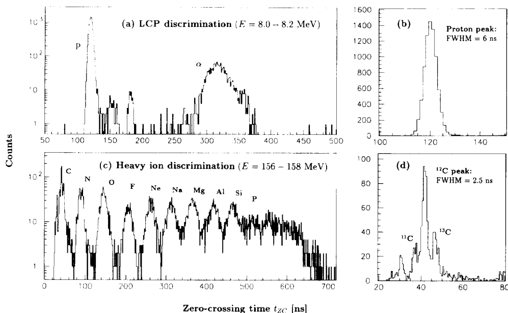
Fig. 7. Projection of small E bins of Fig. 6 onto the calibrated t_{ZC} scale: (a) and (b) projections of Fig. 6a, E = 8.0 – 8.2 MeV, (c) and (d) projections of Fig. 6b, E = 156 – 158 MeV.
