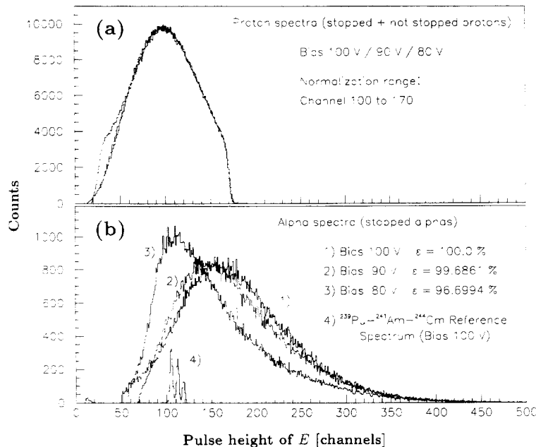
Fig. 10. Pulse-height spectra of LCP produced in the reaction 150 MeV ^{36}Ar + Ni at \theta_{lab} = 110^\circ , measured with a shaping-time constant \tau_E = 0.5 \mu s for different bias voltages: (a) Pulse-height spectra of protons, (b) Pulse-height spectra of alpha particles. The peak shifts and the shape variations of the alpha spectra result from the energy- and bias-dependent ballistic deficit. The counting efficiency \epsilon is nearly constant.
