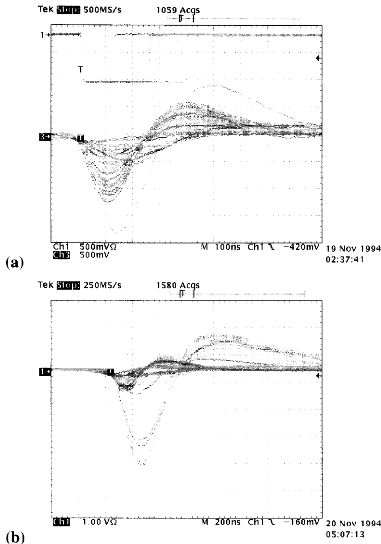
Fig. 3. Typical bipolar signals at the inspection point (see Fig. 2) measured with a digitizing oscilloscope: (a) p and \alpha signals from 150 MeV ^{36}\text{Ar} + \text{Ni} , detector at \theta_{\text{lab}} = 110^\circ ; (b) p, \alpha , and heavy-ion signals from 510 MeV ^{36}\text{Ar} + [\text{Ag} + \text{Au}] , detector at \theta_{\text{lab}} = 25^\circ . The bipolar shaping is performed with two successive timing-filter amplifiers, ORTEC 474/579, both operated with time constants of \tau_{\text{diff}} = 100 \text{ ns} and \tau_{\text{int}} = 50 \text{ ns} .
