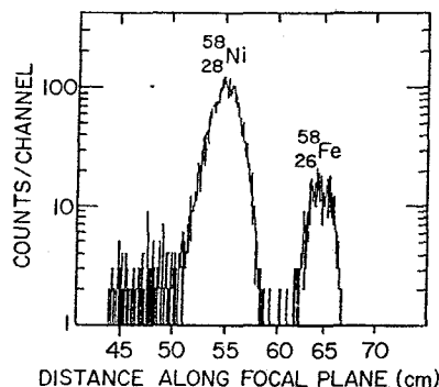
Fig. 5. Separation between two isobaric ions, ^{58}\text{Ni} and ^{58}\text{Fe} at 350 MeV kinetic energy obtained in the focal plane of the gas-filled split-pole spectrograph. The pressure of the gas (nitrogen) is 14 Torr. The isobaric ions accelerated simultaneously with a charge state of 18^+ , were scattered off a Au target at 3^\circ prior to their analysis in the spectrograph (see text).
