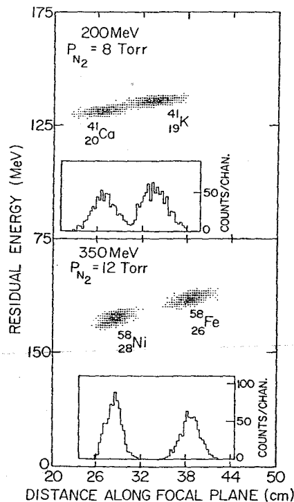
Fig. 14. Calculated two-dimensional spectra of residual energy vs position along the focal plane for isobaric pairs ^{41}\text{K} – ^{41}\text{Ca} (top) and ^{58}\text{Ni} – ^{58}\text{Fe} (bottom) at the specified energies. The inserts show the projection of the groups along the focal plane axis. The plots reproduce the physical separation along the focal plane and the difference in residual energy of the isobaric ions due to the difference of the energy losses in the gas. Within each group, a correlation between residual energy and position can be seen. The plots can be compared to the experimental spectra in figs. 5 and 8.
