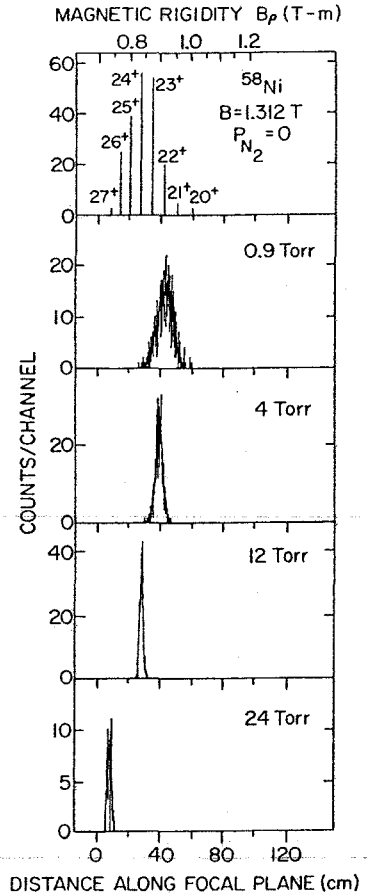
Fig. 11. Position spectra calculated by Monte Carlo simulation, as explained in text, for ^{58}\text{Ni} ions in the gas-filled split-pole magnetic spectrograph. Note the shift in the position of the centroid between the spectrum in vacuum ( P=0 ) and at 0.9 Torr, corresponding respectively to the mean charge state of the ions after passing through the Mylar entrance foil of the magnet and the mean charge state in the gas. At higher gas pressures, the centroid of the group is moving towards smaller magnetic rigidities because of the energy loss in the gas. A similar behavior is observed in the experimental spectra in fig. 3.
