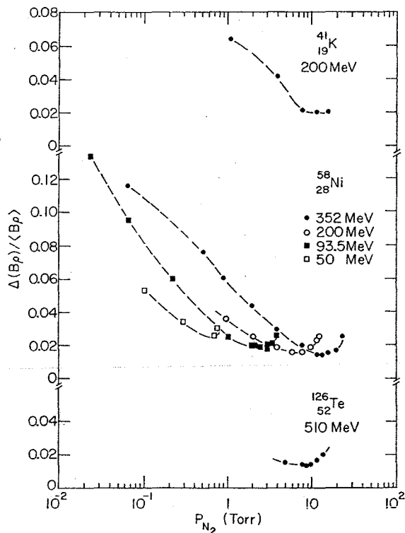
Fig. 4. Empirical dependence of the magnetic rigidity resolution \Delta(B\rho)/\langle B\rho of the spectrum in the focal plane of the gas-filled split-pole magnetic spectrograph as a function of the gas pressure (nitrogen) for ^{41}\text{K} , ^{58}\text{Ni} , and ^{126}\text{Te} ions at the specified incident energies. The ordinate represented the ratio \Delta(B\rho)/\langle B\rho of the full width at half-maximum of the focal plane spectra to the average magnetic rigidity. The dashed line connect the experimental points to guide the eye.
