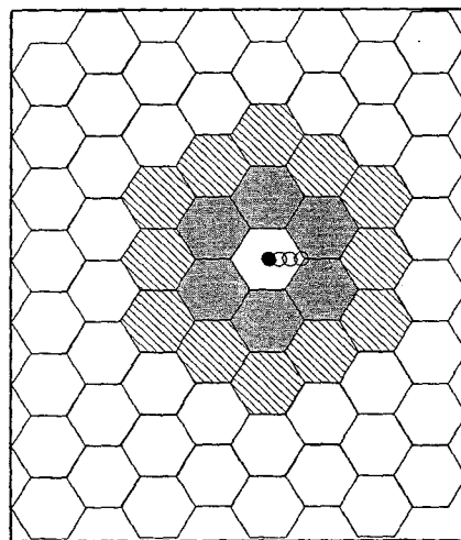
Fig. 5. Position of the illuminated detector within one TAPS-block consisting of 64 \text{BaF}_2 modules. The full and open circles mark the chosen size and positions of the beam spot.
