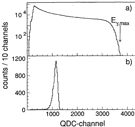
Fig. 6. (a) Response of TAPS to the tagged bremsstrahlung spectrum. E_{\gamma,\text{max}} indicates the maximum tagged photon energy. (b) Response of TAPS to tagged photons with energies of \approx 258 MeV selected by coincidence with the corresponding electrons.
