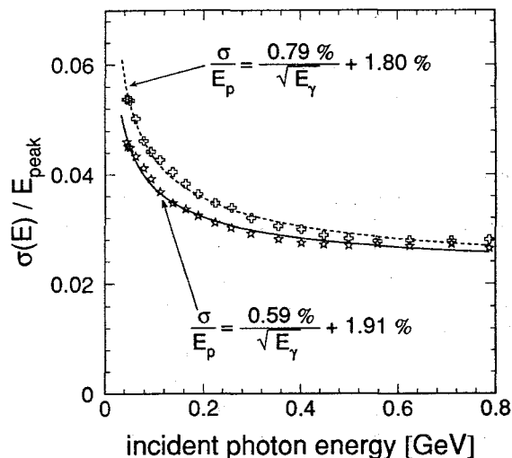
Fig. 11. Measured energy resolution \sigma/E_{\text{Peak}} of the total light output (integration gate 2 \mu\text{s} ), stars, and the fast scintillation component (integration gate 50 ns), crosses, as a function of the incident photon energy. The values are extrapolated to zero incident energy width. The energy dependence has been parametrized by \sigma/E = AE^{-1/2} + B as shown in the figure.
