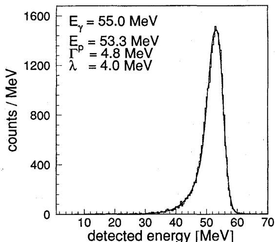
Fig. 10. Experimental line shape measured at E_\gamma = 55 MeV compared to the fitted analytical response function. The values of the fit parameters (see text) are shown in the figure.
