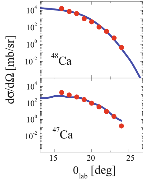
Fig. 8. Angular distributions for the elastic and for the one-neutron stripping channels. Symbols refer to experimental data while solid lines give the theoretical predictions from the semiclassical GRAZING model.
