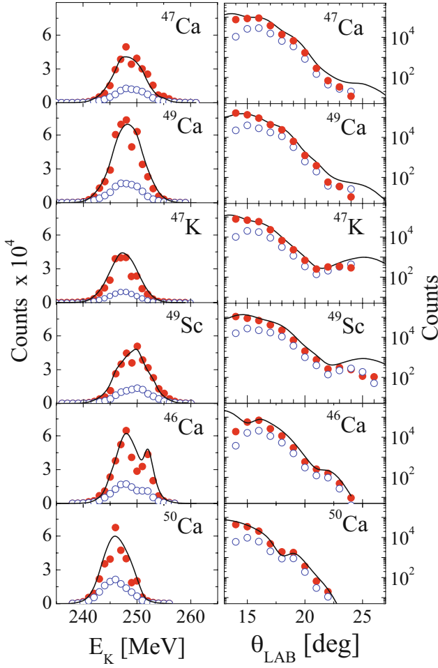
Fig. 7. Kinetic energy (left) and dispersion angle \theta_{lab} (right) distributions of the \pm 1n , \pm 1p \pm 2n channels of the reaction ^{48}\text{Ca} on ^{64}\text{Ni} at E_{lab} = 270 MeV, as calculated by the GRAZING model [7] (solid lines). The open circles give the corresponding simulated distributions obtained at the focal plane of the PRISMA spectrometer, while the full circles represent the same distributions corrected by the factors f(E_K, \theta_{lab}) , shown in fig. 6 (see text for details).
