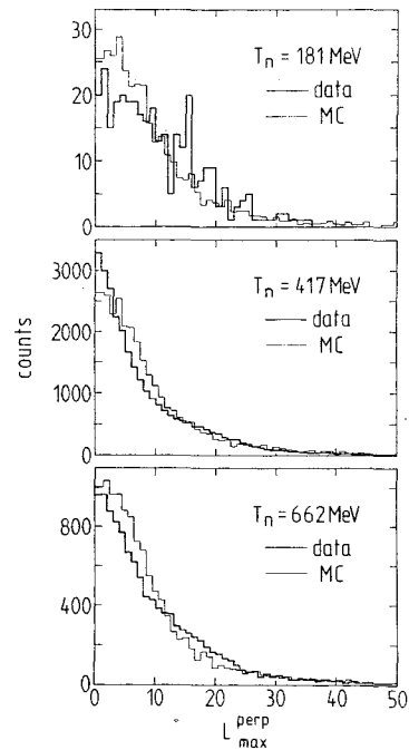
Fig. 13. Distribution of the maximum shower length projected onto a plane perpendicular to the incident neutron, L_{\text{max}}^{\text{perp}} , for tagged neutrons of T_n = 181, 417 and 662 MeV. For comparison HERMES/HETC predictions are included.
