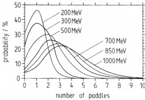
Fig. 14. Simulated probability distribution of the paddle multiplicity resulting from monoenergetic neutrons impinging on LAND with indicated energies.
