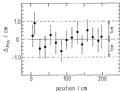
Fig. 6. Deviation of the measured position of light production from the real position for an arbitrarily selected neutron detector paddle. Cosmic radiation was used for this measurement.
