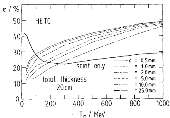
Fig. 2. Calculated efficiencies of an iron/scintillator structure of 2 \times 2 m area and a depth of 20 cm as a function of neutron kinetic energy. Various layer thicknesses d (with d(\text{Fe}) = d(\text{scint}) ) are considered. The thick solid line is for pure scintillator material.
