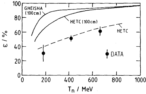
Fig. 9. Measured efficiency of the test setup for tagged neutrons of T_n = 181, 417 and 662 MeV. The dashed curve is the result of a Monte Carlo simulation using the HERMES/HETC code for the same geometry. The efficiency of the full size detector (100 cm thick) is also shown as predicted by GEANT/GHEISHA and HERMES/HETC.
