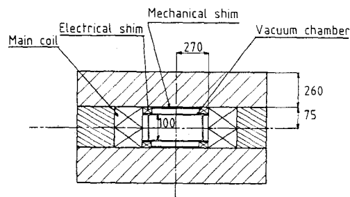
Fig. 5. Vertical cross section of the analysing magnet (DA). Distances are given in millimeters.
