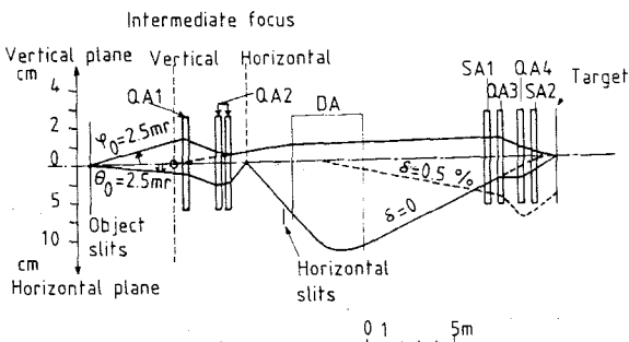
Fig. 3. Beam profile along the incident beam line, for nominal tuning (no kinematics). Beam emittance is assumed to be 5 \pi mm mrad in both planes, and object size to be 4 \times 4 mm 2 .
