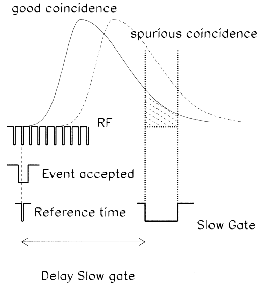
Fig. 2. Sketch of the slow gate timing. The “event accepted” signal, produced by the trigger, enables one RF signal. This signal is used as reference time to generate all gates. The dashed region shows the SLOW integration region of a signal produced by a good coincidence. One can note the difference with the charge integrated with the same gate for a signal produced in a different burst (dashed signal spurious coincidence). The time scale of the real experiment has been not respected to better evidence the effect.
