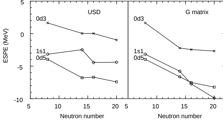
Figure 4: Effective single-particle energies for the oxygen isotopes.
