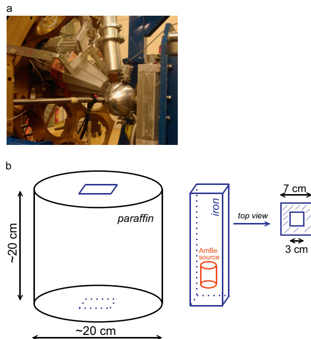
Fig. 1. Upper panel: The experimental set-up consisting of two AGATA triple clusters and one 3.5'' × 8'' cylindrical LaBr 3 :Ce scintillation detector. Lower panel: schematic representation of the Am–Be–Fe source.
