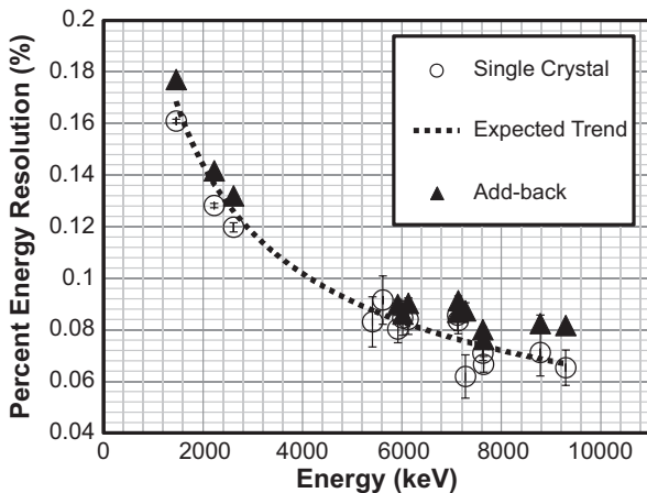
Fig. 3. Relative energy resolution of the AGATA detectors is given for the Am–Be–Fe source data. The data for the best performing single detector are shown by empty black circles. The black triangles represent instead the energy resolution for the add-back procedure, performed among all crystals that fired in each event. The experimental data follow the expected E^{-1/2} trend (indicated by the dashed black line).
