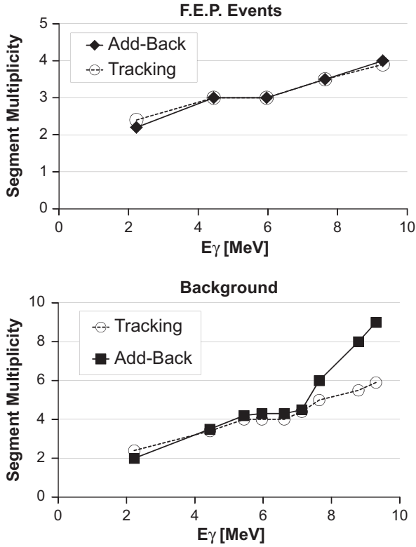
Fig. 7. Segments multiplicity as a function of gamma energy for FEP and background events. Results for gamma-ray tracking and standard “add-back” are compared. The centroids of each distribution are plotted with empty circles and black squares respectively. Error bars are smaller than symbol size.
