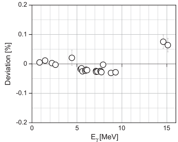
Fig. 5. Deviation of the measured energies from the tabulated energy for each gamma line of the Am–Be–Fe source and for the 4.4 and 15.1 MeV gammas from the in-beam test. If not displayed, error bars are smaller than the symbol size.
