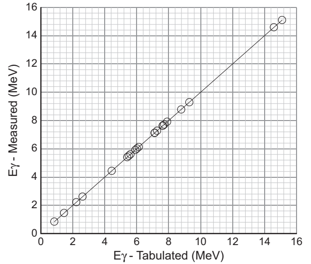
Fig. 4. Tabulated energy versus measured energy for gamma lines of the Am–Be–Fe source and for the 4.4 and 15.1 MeV gammas from the in-beam test.
