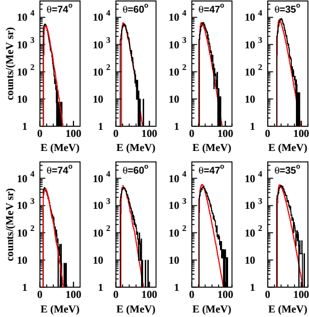
Fig. 1. Upper row — global (simultaneous for different detection angles) moving source fit for the experimental \alpha -particle spectra at four different angles for the Ni + Zn at 400 MeV. Lower row — the same as in upper row, but for the Ni + Zn at 500 MeV.
