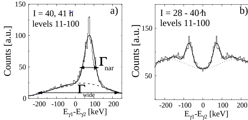
Fig.1. Panel (a): projection on the E_{\gamma_1}-E_{\gamma_2} axis of the E2 strength function for two consecutive E2 \gamma -rays, calculated microscopically for the levels 11–100 at spin I = 40, 41\hbar for ^{163}\text{Er} [9]. The full drawn line represents the analytic two-component function containing a wide and a narrow Gaussian component of width \Gamma_{\text{wide}} and \Gamma_{\text{nar}} , respectively. Panel (b): projection on the E_{\gamma_1}-E_{\gamma_2} axis of a spectrum microscopically calculated for multiple steps of E2 decay, for the levels 11–100 of ^{163}\text{Er} , in the spin range 28 to 40 \hbar . The full drawn line is the parametrized spectrum for multiple steps, with \Gamma_{\text{rot}} = 180 keV and \Gamma_{\text{nar}} = 44 keV, while the dashed line has no narrow component and a width \Gamma_{\text{rot}} = 150 keV.
