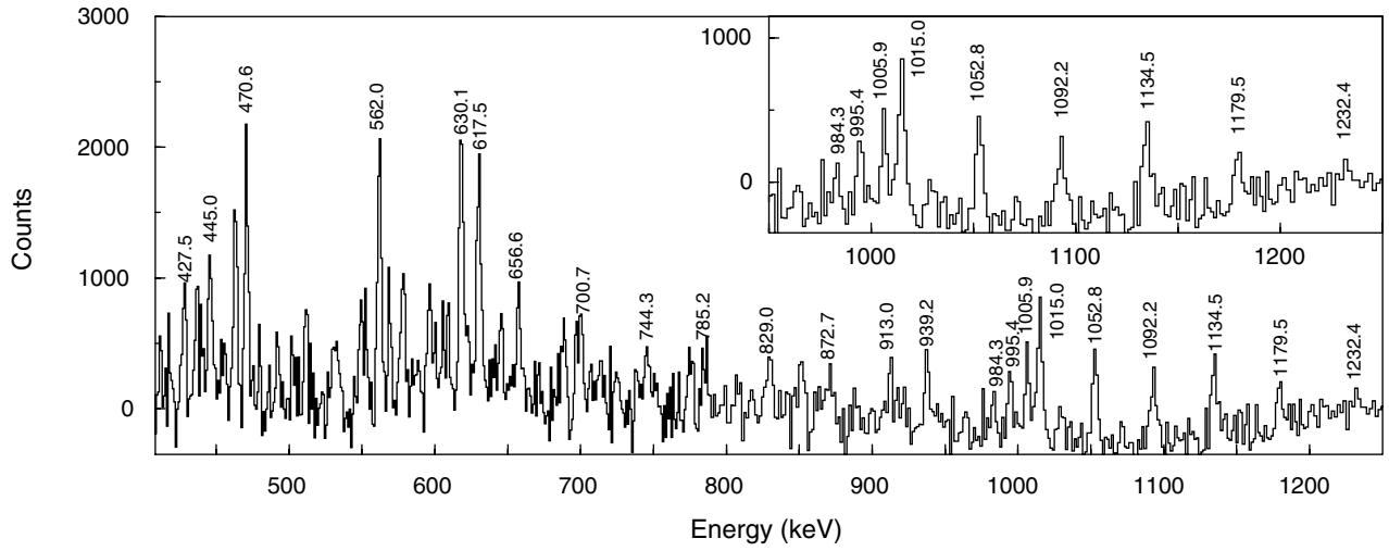
Fig. 10. Spectrum showing the ND band, X5, obtained from the 3D-coincidence cube using a sum of double gates on the transitions 1015.0, 1052.8, 1092.2, 1134.5, 1179.5, and 1232.4 keV. The inset shows an expansion of the high-energy part of the spectrum.
