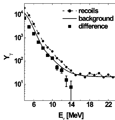
FIG. 3. The spectra of high-energy \gamma rays for three different conditions: recoils and background corresponding to the gates shown in Fig. 2 and the difference of these two spectra shown with filled squares.
