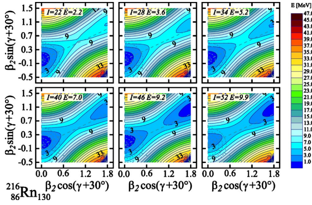
FIG. 8. (Color online) The ^{216}\text{Rn} potential energy maps calculated using the LSD model. As one can see, this approach predicts for the ^{216}\text{Rn} nucleus an equilibrium shape (cf. the minima of the potential energy) which is approximately spherical up to the spins around I=40\hbar . At I=40\hbar , the fission barrier is about 3 MeV high, so that for I\geq 40\hbar the fission decay mode is expected to dominate. Note that the only evolution with spin is the decreasing in the barrier height and no Jacobi transition is expected in this nucleus according to the calculations.
