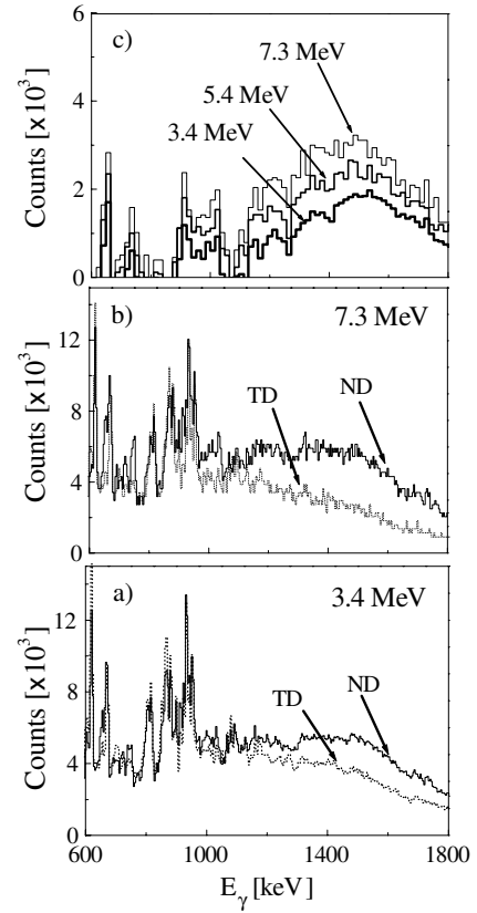
Fig. 5. Spectra of ^{143}\text{Eu} collecting the entire decay flow (ND) and the triaxial contribution only (TD), gated by high-energy transition with \langle E_{\gamma} \rangle = 3.4 (panel a)) and 7.3 MeV (panel b)). The intensity of the E2 bump observed in the ND spectra, obtained as a difference between the ND and TD spectra and normalized to the intensity of the 553 keV low-spin spherical transition, is shown in the top part (panel c)) of the figure. (Adapted from [8].)
