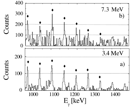
Fig. 3. Spectra of the SD yrast of ^{143}\text{Eu} , gated by high-energy \gamma -rays with average energies \langle E_\gamma \rangle = 3.4 (panel a)) and 7.3 MeV (panel b)). The spectra are normalized to the intensity of the low-spin 917 keV line, with the gating condition \langle E_\gamma \rangle = 7.3 MeV. The diamonds indicate the SD lines used to calculate the increase of the yrast intensity. (Adapted from [8].)
