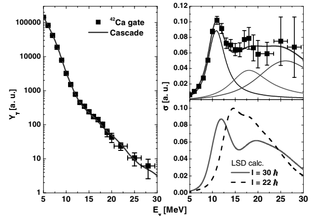
Fig. 2. Left: spectrum of the \gamma -rays from the decay of the GDR built in hot ^{46}\text{Ti} in coincidence with the discrete transitions in the residual nucleus ^{42}\text{Ca} , together with the Cascade calculations assuming 3-Lorentzian GDR strength function with E_{\text{GDR}} = 10.8, 18 and 26 MeV. Upper right: experimentally obtained GDR absorption cross-section and the GDR strength function used in Cascade calculations. Bottom right: thermal shape fluctuation predictions based on potential energies from the LSD model calculations for I = 22\hbar and I = 30\hbar .
