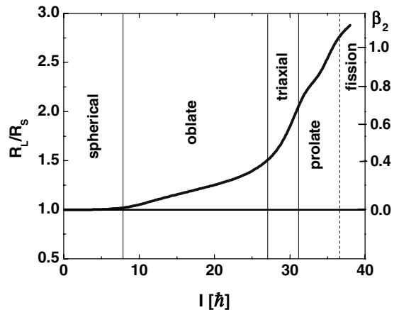
Fig. 1. Long-to-short axis ratio and the \beta_2 parameter for the equilibrium deformation as a function of spin, obtained from the LSD model calculations for ^{46}\text{Ti} .
