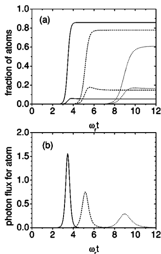
FIG. 2. (a) Fraction of atoms in |c, 1\rangle (upper curves) and in |b, -1\rangle (lower curves) vs \omega t , for G=10\omega_r , \gamma_1=\gamma_2=0.3\omega_r and \alpha=N_c/N_b=0.1 (continuous lines), \alpha=0.5 (dashed lines), and \alpha=1 (dotted lines). (b) photon flux for atom, 2\kappa|a|^2/N_b=G|S_1+S_2|^2 , for \alpha=0.1 (continuous line), \alpha=0.5 (dashed line), and \alpha=1 (dotted line).
