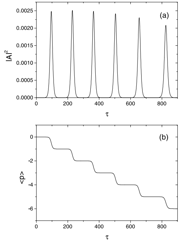
Fig. 3. Sequential SF regime of CARL: (a) |A|^2 and (b) \langle p \rangle vs. \tau , for \rho = 2 , \delta = 0.5 , \kappa = 10 , and the same initial conditions of Fig. 2.
