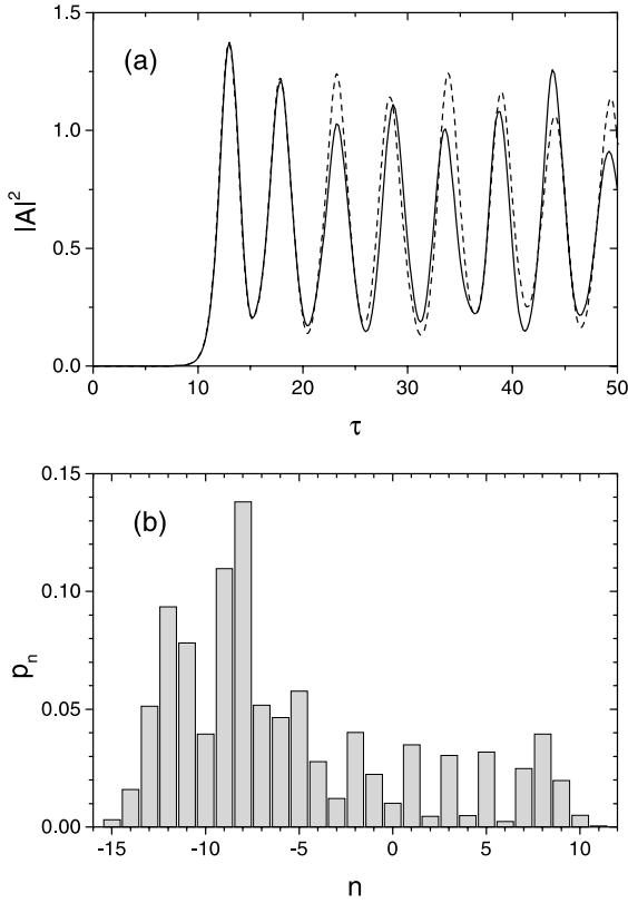
Fig. 1. Classical limit of CARL for \rho \gg 1 in the case \kappa = 0 : (a) |A|^2 vs. \tau as obtained from the classical equations (1)–(3) (---) and from the quantum equations (7) and (8) for \rho = 10 (—); (b) population level p_n vs. n at the occurring of the first maximum of |A|^2 , at \tau = 12.4 . The other parameters are \delta = 0 and A(0) = 10^{-4} .
