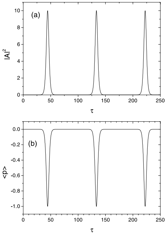
Fig. 2. Quantum limit of CARL for \rho < 1 in the case \kappa = 0 : (a) |A|^2 and (b) \langle p \rangle vs. \tau , for \rho = 0.2 , \delta = 5 , A(0) = 10^{-5} and the atoms initially in the state n = 0 . We note that \langle p \rangle = -(\rho/2)(|A|^2 - |A(0)|^2) .
