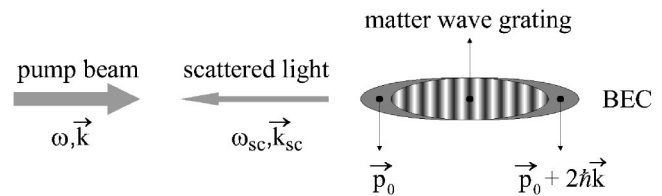
FIG. 1. Schematics of superradiant light scattering from a Bose-Einstein condensate. An elongated BEC with momentum \vec{p}_0 is illuminated by a far-off-resonant laser beam ( pump beam ) with frequency \omega and wave vector \vec{k} directed along its axial direction. After backscattering of photons with \vec{k}_{sc} \approx -\vec{k} and the subsequent recoil of atoms, a matter-wave grating forms, due to the quantum interference between the two momentum components \vec{p}_0 and \vec{p}_0 + 2\hbar\vec{k} of the wave function of the condensate. The effect of this grating is to further scatter the incident light in a self-amplifying process.
